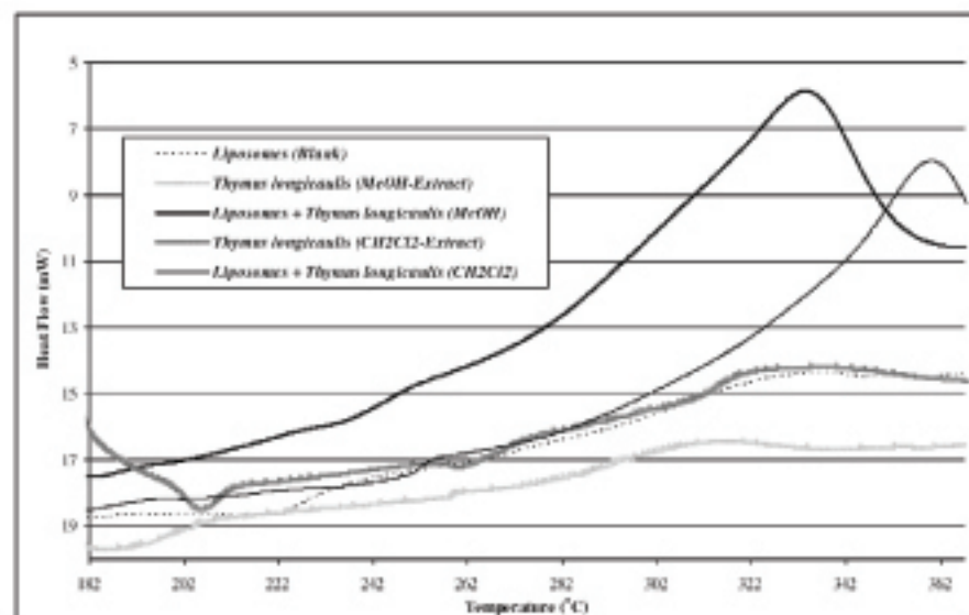
FIGURE 6. DSC oxidation (DSC-heat flow/temperature) of Thymus longicaulis pure extracts and encapsulated in liposomes. Values are means of triplicate determinations.
