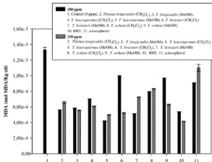
FIGURE 2. Malondialdehyde (MDA) concentration in sunflower oil after UV accelerated method with various concentrations of pure extracts (100 and 150 ppm). Values are means of triplicate determinations.
