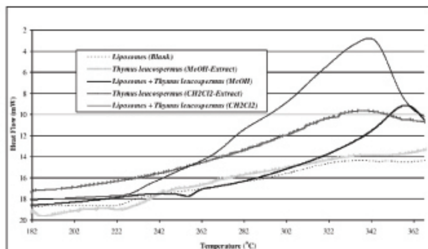
FIGURE 3. DSC oxidation (DSC-heat flow/temperature) of Thymus leucospermus pure extracts and encapsulated in liposomes. Values are means of triplicate determinations.
