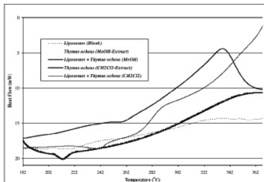
FIGURE 5. DSC oxidation (DSC-heat flow/temperature) of Thymus ocheus pure extracts and encapsulated in liposomes. Values are means of triplicate determinations.
