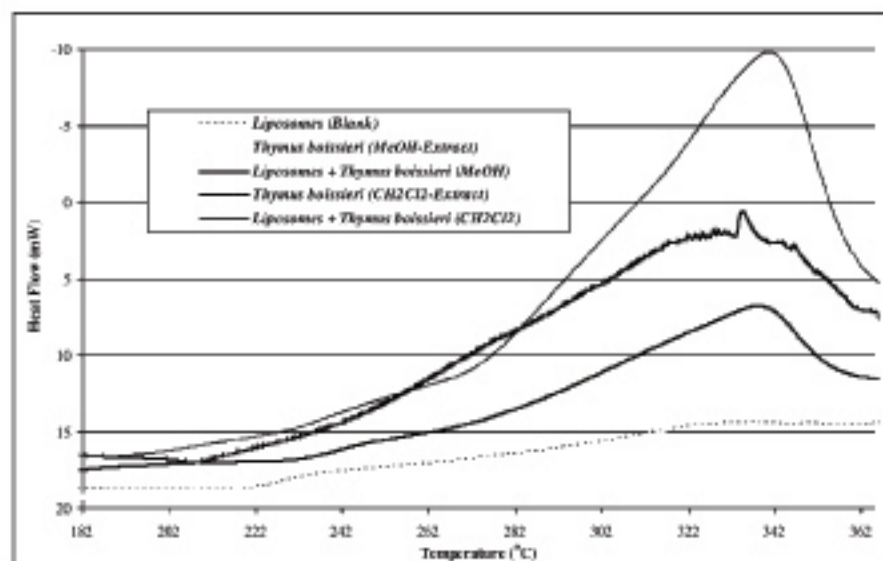
FIGURE 4. DSC oxidation (DSC-heat flow/temperature) of Thymus boissieri pure extracts and encapsulated in liposomes. Values are means of triplicate determinations.
